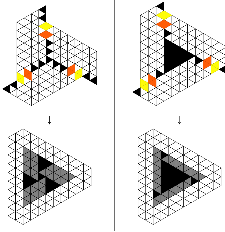
Figure 7: Pinwheel and hexagon figures for (s, t, n, \mu) = (2, 0, 4, 3) in Lemma 8. The left column is associated to \mathcal{E}_{s,0}^\mu(n) and the right column is associated to \mathcal{D}_{s-1,0}^{\mu+3}(n-1) . Note that the region to be tiled is the same in both cases (after removing all regions of forced tilings).
