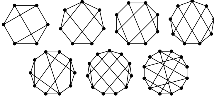
Figure 7: Circular embedding of the Laman graphs with maximal Laman numbers for 6 \leq n \leq 12 . Note that these are the same graphs that are displayed in Figure 5.
